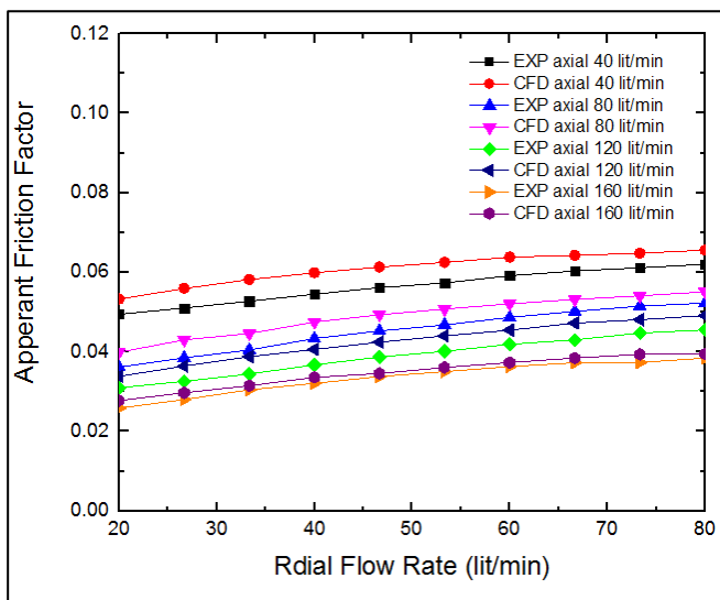
Fig. 14 Comparison between the experimental and numerical apperant friction factor with radial flow rate.
